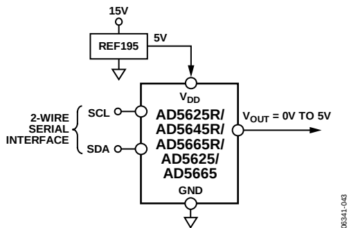
Figure 73. REF195 as Power Supply to the AD56x5R/AD56x5
