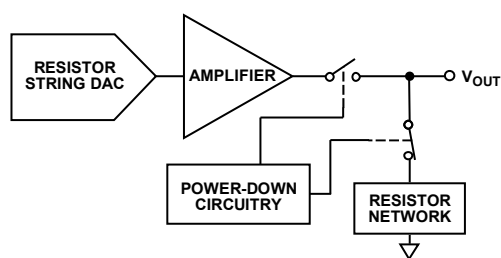
Figure 69. Output Stage During Power-Down
