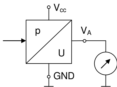
3-wire connection (standard)
