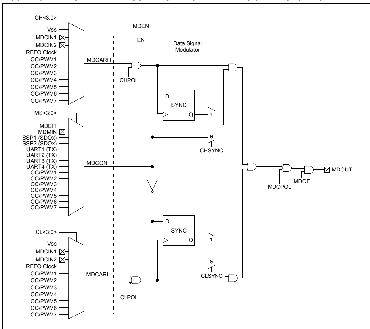
FIGURE 20-1: SIMPLIFIED BLOCK DIAGRAM OF THE DATA SIGNAL MODULATOR
