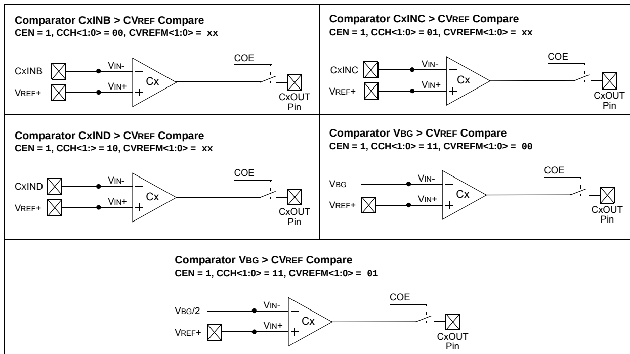
FIGURE 30-4: INDIVIDUAL COMPARATOR CONFIGURATIONS WHEN CREF = 1 AND CVREFP = 1
