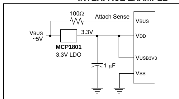
FIGURE 19-2: BUS-POWERED INTERFACE EXAMPLE
