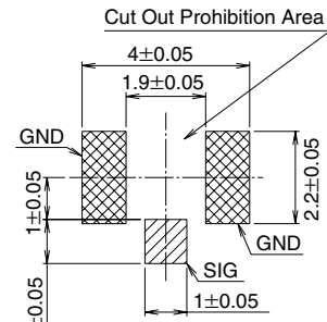
Recommended PCB mounting pattern
