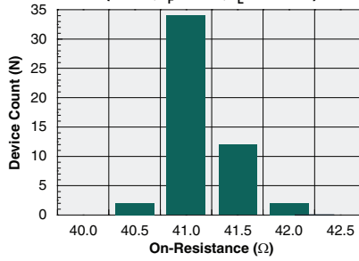
Typical On-Resistance Distribution (N=50, I F =2mA, I L =100mA)
