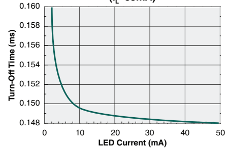
Typical Turn-Off Time vs. LED Forward Current (I L =55mA)
