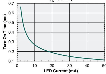
Typical Turn-On Time vs. LED Forward Current (I L =55mA)
