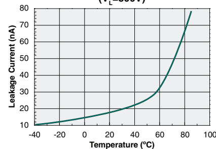
Typical Leakage Current vs. Temperature (V L =800V)
