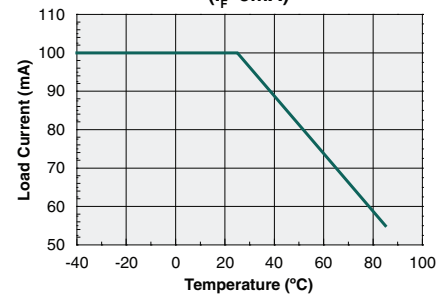
Maximum Load Current vs. Temperature (I F =5mA)
