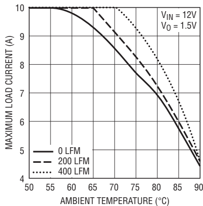
Figure 11. No Heatsink
