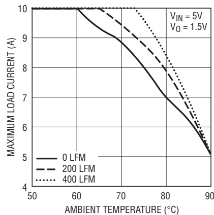
Figure 9. No Heatsink
