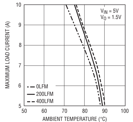
Figure 10. BGA Heatsink
