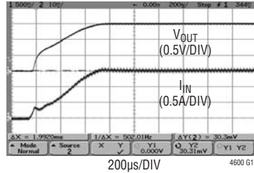
Start-Up, I_{OUT} = 10A (Resistive Load)
