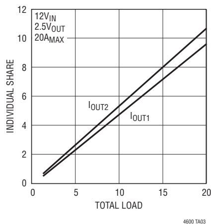
Current Sharing Between Two LTM4600 Modules
