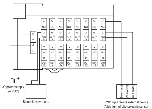
GX-ID3228 (PNP)
