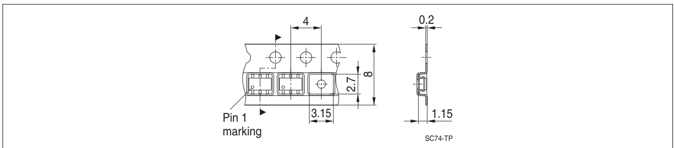
Figure 11 Tape Loading
