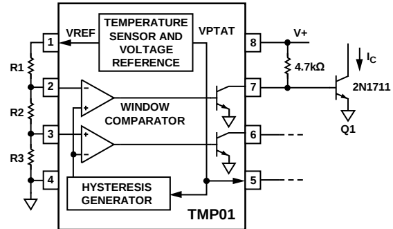
Figure 22. An External Resistor Minimizes Self-Heating
