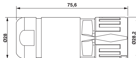
Dimensioned drawing
