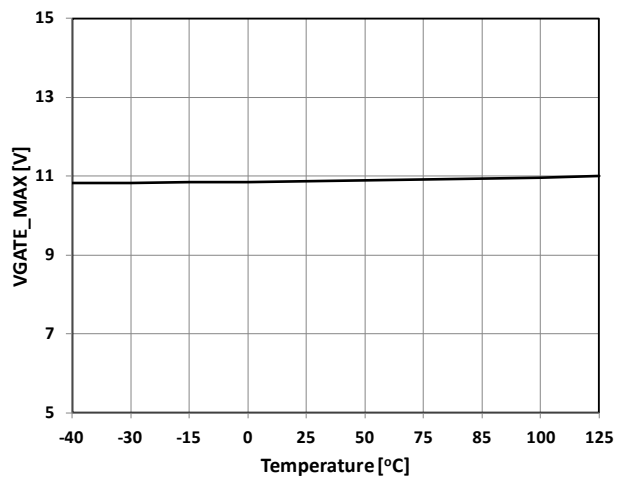
Figure 15. V_{GATE\_MAX}
