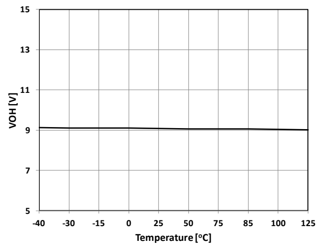
Figure 16. V_{OH}
