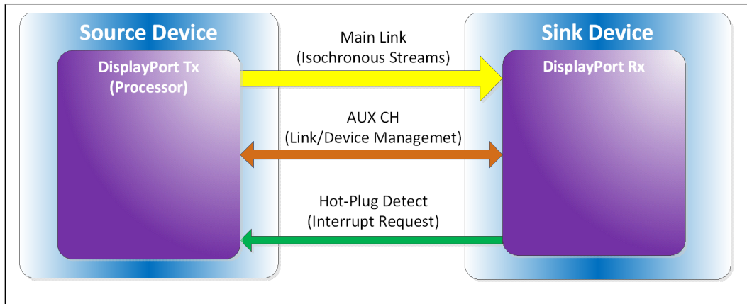
Figure 2-7. DisplayPort* Overview
