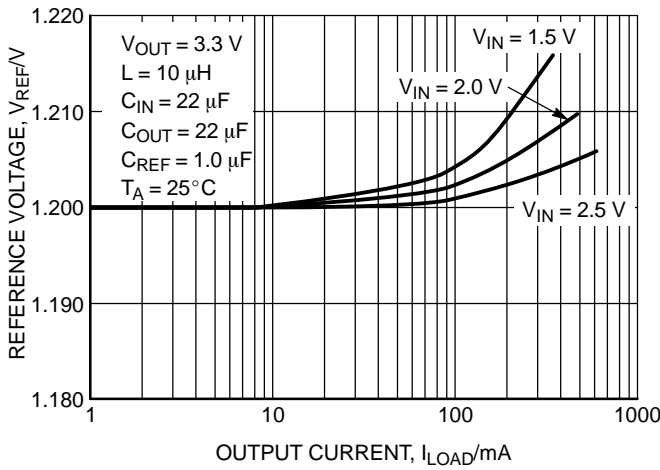
Figure 2. Reference Voltage vs. Output Current
