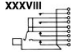
Double closed circuit. Isolated switching—Two “make” circuits.
