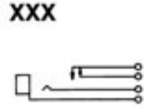
Single open circuit—“make” before “break”. (J11).
