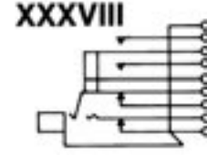
Double closed circuit. Isolated switching—Two “make” circuits.
