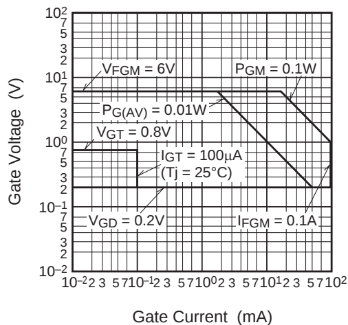
Gate Characteristics
