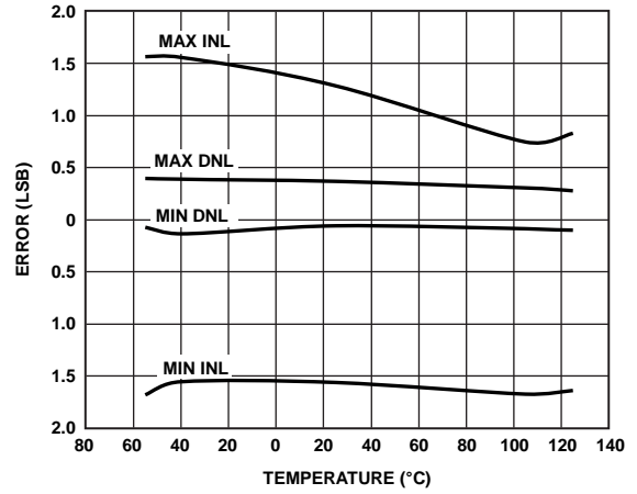
Figure 7. INL and DNL Error vs. Temperature
