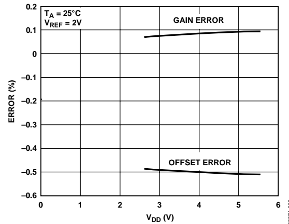
Figure 8. Offset Error and Gain Error vs. V_{DD}
