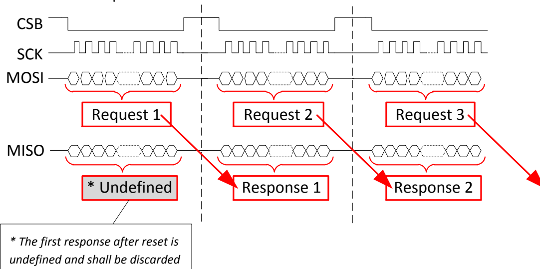
Figure 14. SPI Protocol
