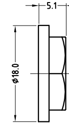
PLASTIC NUT
