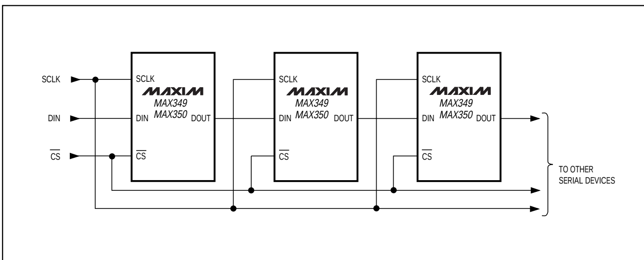
Figure 5. Daisy-Chained Connection
