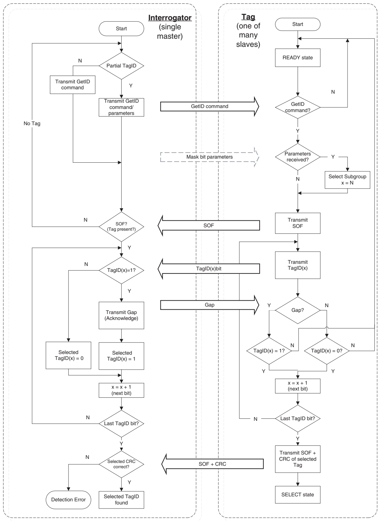
Figure 6-1. Anticollision Loop
