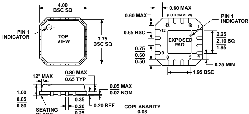
COMPLIANT TO JEDEC STANDARDS MO-220-VGGC Figure 23. 16-Lead Lead Frame Chip Scale Package [LFCSP_VQ] 4 mm x 4 mm Body, Very Thin Quad (CP-16-4) Dimensions shown in millimeters
