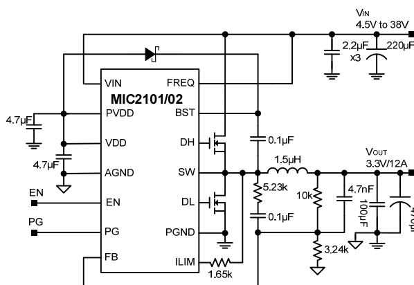
MIC2101/02 Wide Input, Hyper Light Load Buck Converter
