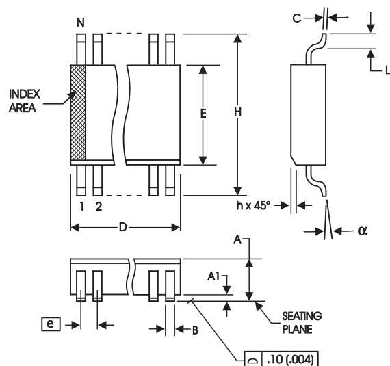
150mil Body, .50mil pitch
