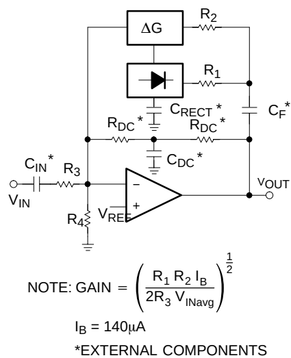
Figure 7. Basic Compressor
