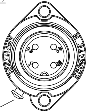
MALE RECEPTACLE
