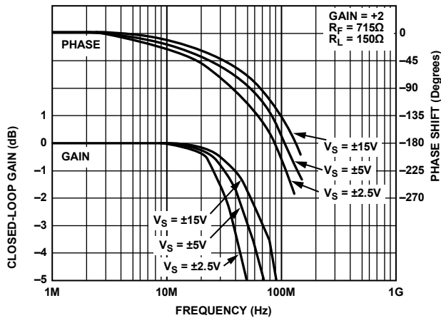
Figure 53. Closed-Loop Gain and Phase Shift vs. Frequency, G = +2 , R_L = 150\Omega , R_F = 715\Omega
