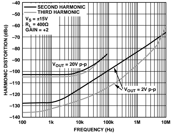
Figure 21. Harmonic Distortion vs. Frequency ( R_L = 400\ \Omega )
