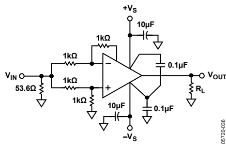
Figure 42. Common-Mode Rejection
