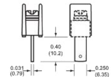
09 0.250" QC short
