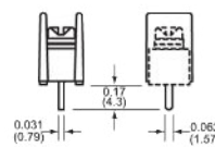
08 Printed Circuit
