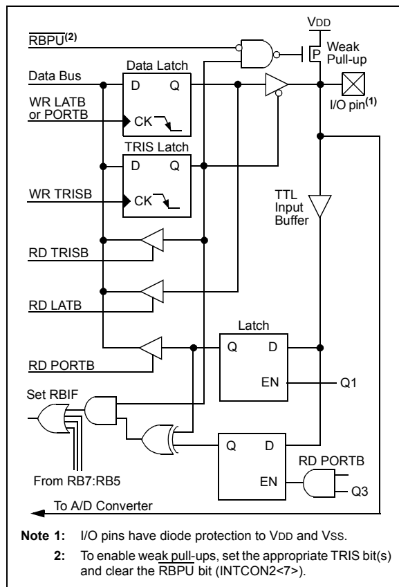
FIGURE 10-8: BLOCK DIAGRAM OF RB4 PIN
