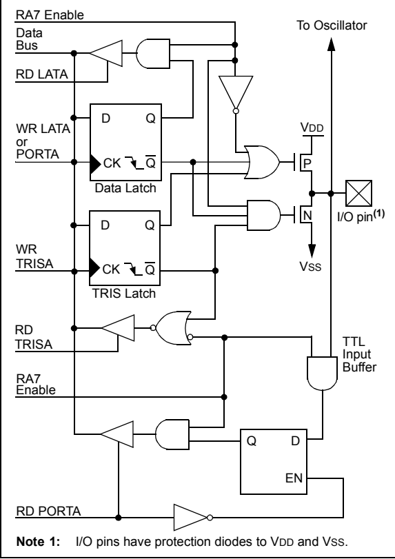
FIGURE 10-5: BLOCK DIAGRAM OF RA7 PIN
