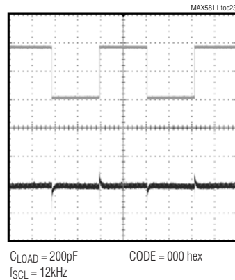
DIGITAL FEEDTHROUGH
