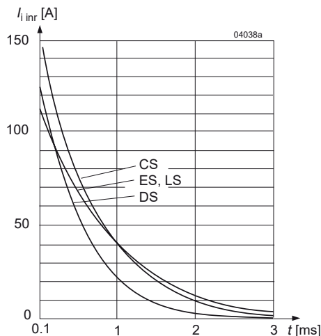
Fig. 3 Typical inrush current versus time at V_{\text{i max}} , R_{\text{ext}} = 0 \Omega . For AS, BS, FS, and for application-related values, use the formula in this section to get realistic results.
