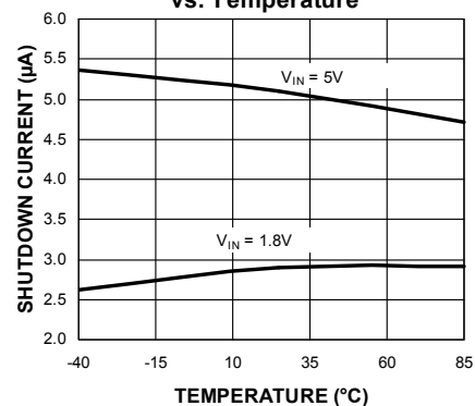
V_{\text{IN}} Shutdown Current vs. Temperature
