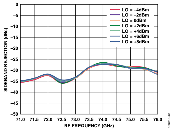
Figure 39. Sideband Rejection vs. RF Frequency at Various LO Powers, I_{FIN} = -8 \text{ dBm} , IF = 2000 \text{ MHz} , LSB
