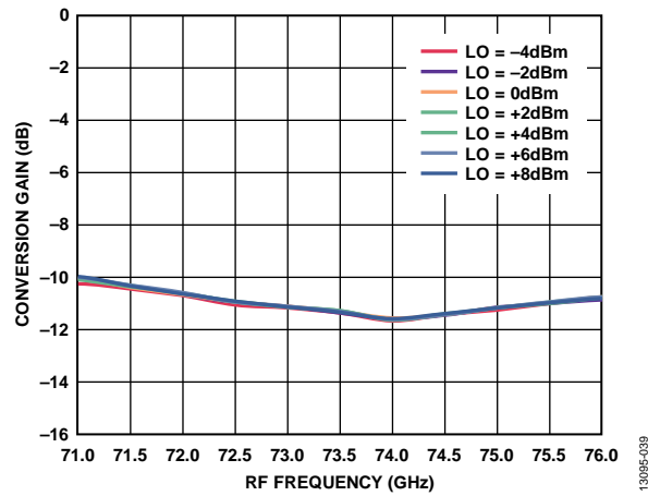
Figure 38. Conversion Gain vs. RF Frequency at Various LO Powers, I_{FIN} = -8 \text{ dBm} , IF = 2000 \text{ MHz} , LSB
