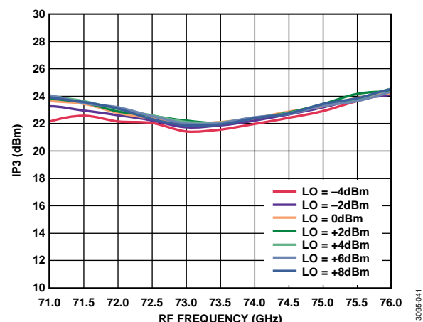
Figure 40. Input IP3 vs. RF Frequency at Various LO Powers, I_{FIN} = 5 \text{ dBm} , IF = 2000 \text{ MHz} , LSB
