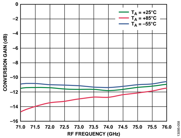
Figure 57. Conversion Gain vs. RF Frequency at Various Temperatures, IF_{IN} = -8 dBm, LO = 2 dBm, IF = 1000 MHz, USB
