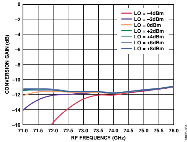
Figure 60. Conversion Gain vs. RF Frequency at Various LO Powers, IF_{IN} = -8 dBm, IF = 1000 MHz, USB
