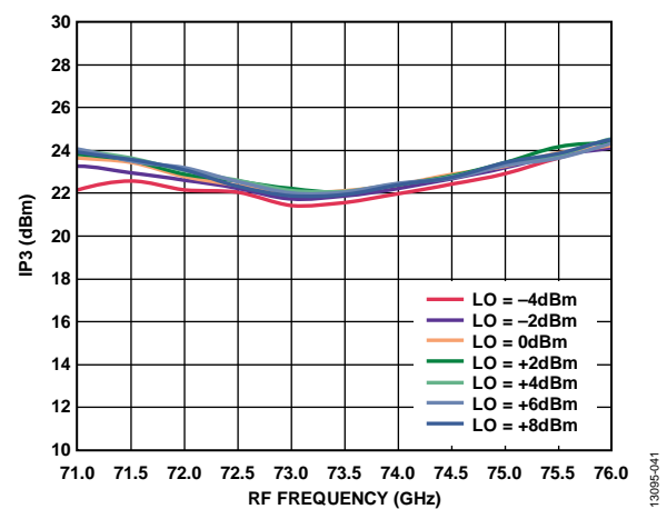
Figure 40. Input IP3 vs. RF Frequency at Various LO Powers, I_{FIN} = 5 dBm, IF = 2000 MHz, LSB
