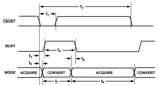
Figure 35. Basic Conversion Timing
