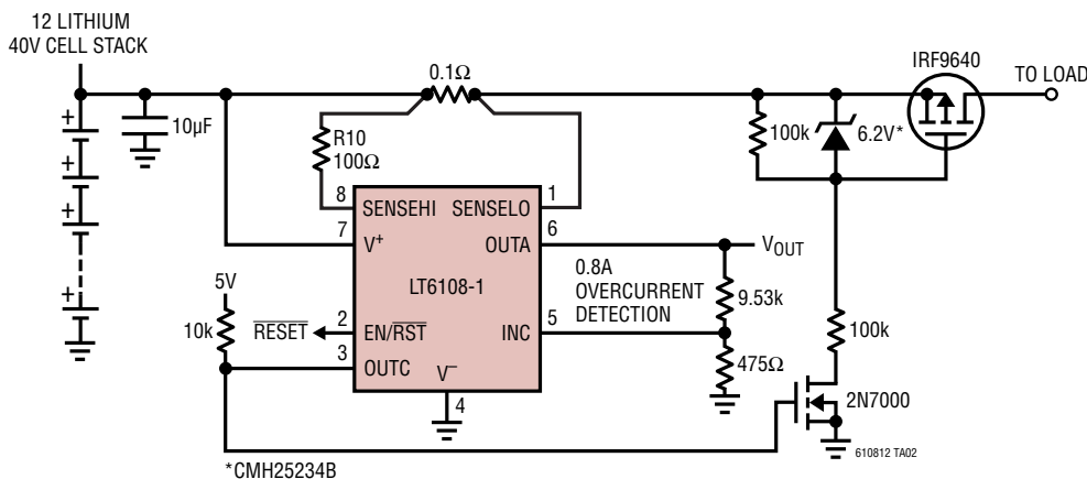
Overcurrent Battery Fault Protection
