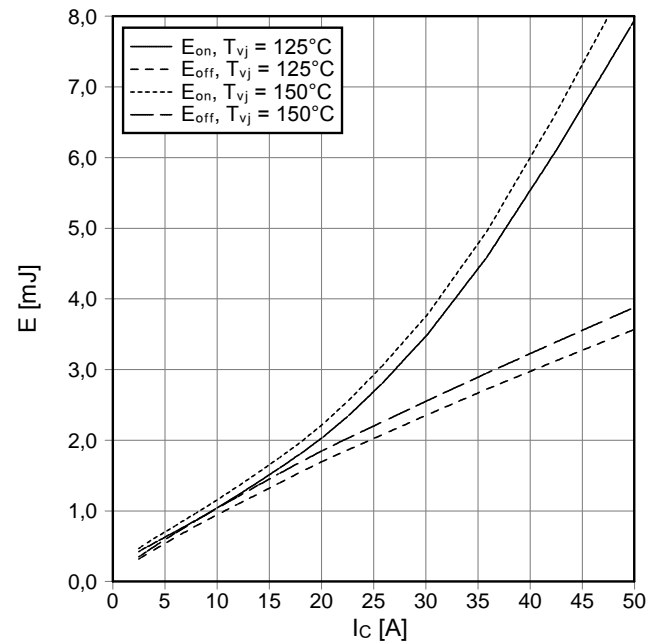
Schaltverluste IGBT-Wechselr. (typisch) switching losses IGBT-inverter (typical) E_{on} = f(I_C), E_{off} = f(I_C) V_{GE} = \pm 15\text{ V}, R_{Gon} = 20\ \Omega, R_{Goff} = 20\ \Omega, V_{CE} = 600\text{ V}
