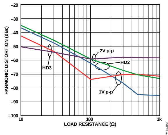
Figure 8. Harmonic Distortion (HD2, HD3) vs. Load Resistance for the High Current Driver—See Figure 54
