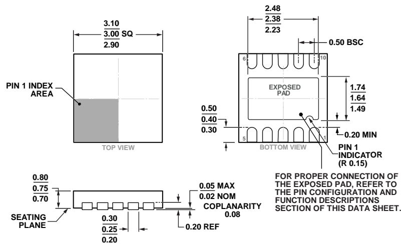
Figure 15. 10-Lead Lead Frame Chip Scale Package [LFCSP_WD] 3 mm x 3 mm Body, Very Very Thin, Dual Lead (CP-10-9) Dimensions shown in millimeters
