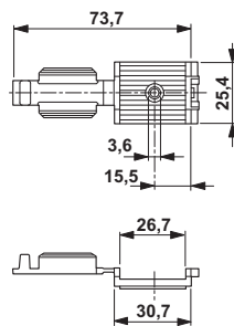
Dimensioned drawing
