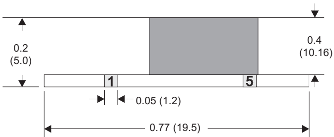
Pin Connections
