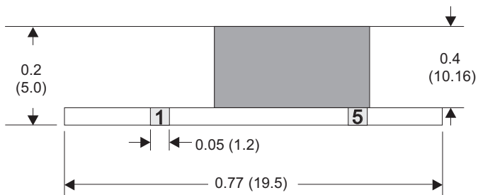
Pin Connections
