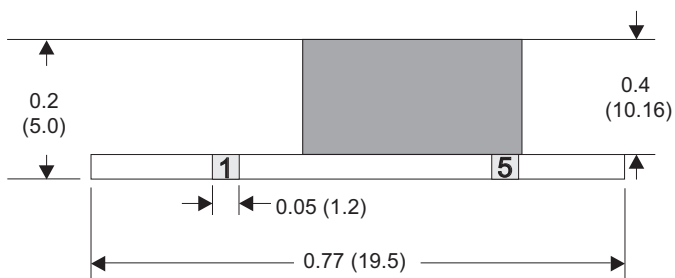
Pin Connections
