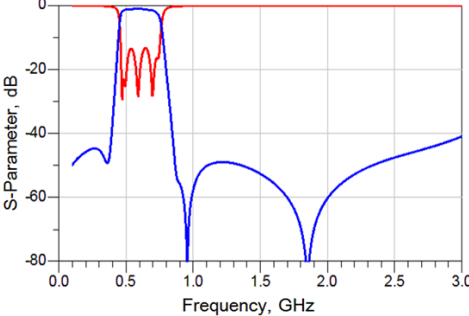
RFBPF3225180C07B1U
