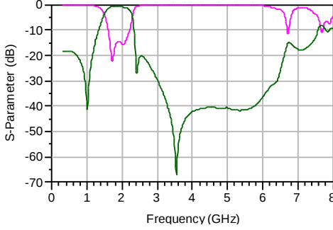
RFBPF3225200Y07B1U
