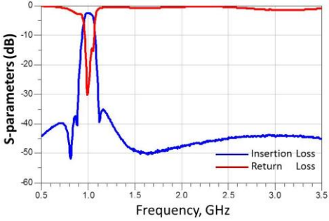
RBBPF3225180Y27B1U
