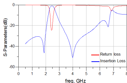
RFBPF2012090A2T
