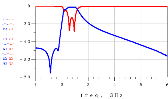
RFBPF1608060K68Q1C
