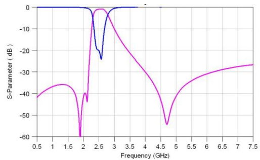
RFBPF2012040AHT
