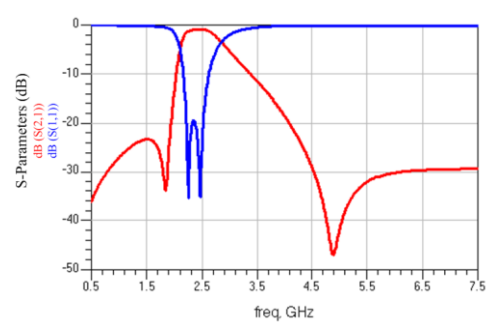
RFBPF1608060ADT
