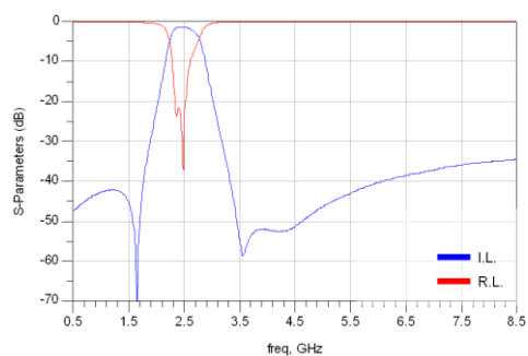
RFBPF1608060AA7M1U
