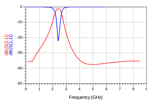
RFBPF1608070AFT
