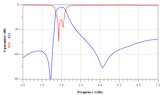
RFBPF2012080AFT
