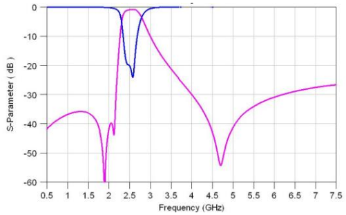
RFBPF2012090AS1T35
