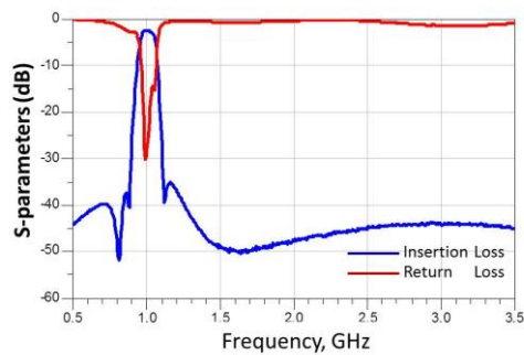
RBBPF3225180Y27B1U
