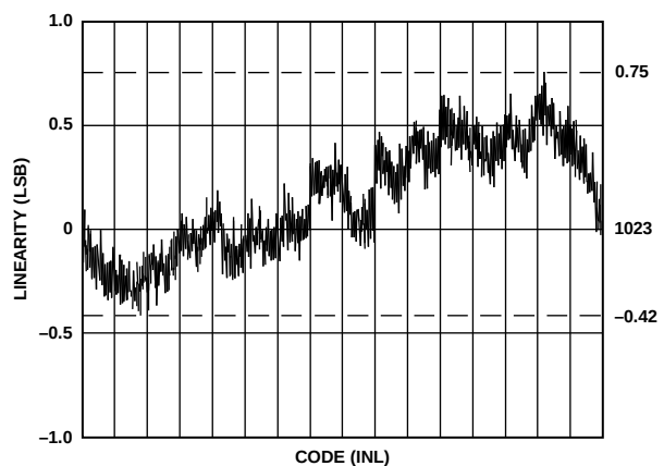
Figure 18. Typical Linearity
